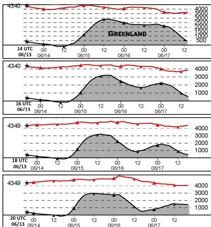
Figure 7: Heights of the four forward trajectories starting on June 13th at 14, 16, 18, and 20 UTC (red curve), and terrain height (black curve) in meters above mean sea level (AMSL). Air mass trajectories start at mid-troposphere over the fire region in Labrador (★).
