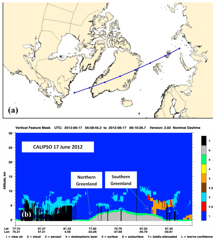
Figure 8: (a) orbit track of CALIPSO on June 17th at about 06 UTC; (b) CALIPSO profile showing aerosols emitted by from eastern Labrador forest fires over southern Greenland at mid-troposphere.
