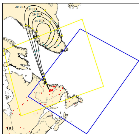
Figure 6: (a) Four day (i.e., 96 hours) forward trajectories of air masses crossing the central Labrador fire region and transporting smoke north to southern Greenland; red dots indicate all fires active during June 2012; the four trajectories start from fire #2 on June 13th at 14, 16, 18, and 20 UTC; yellow (resp. cyan) triangles indicate 00 (resp. 12) UTC of each following day; the last yellow triangles on each forward trajectory correspond to 00 UTC on June 17th. (b) MODIS Aqua imagery (1605 UTC) and active fire hotspots on June 13th; trajectories match the grey smoke plume transport to Labrador Sea. (c) MODIS Terra 14 June 2012 at 15 UTC shows heavy cloud cover over the Labrador Sea. Images courtesy of the MODIS Rapid Response Team, NASA Goddard Space Flight Center.
