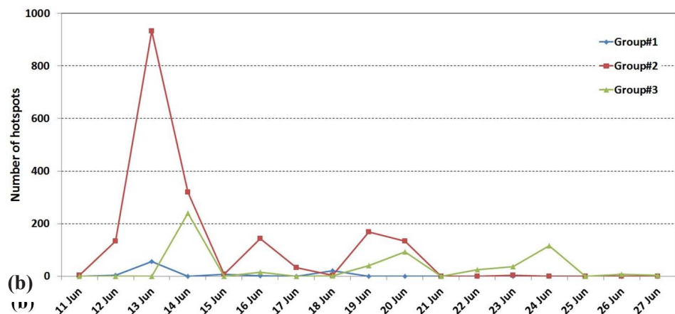
Figure 3: (a) Location of MODIS and AVHRR fire hotspots in Labrador during June-August 2012; (b) Daily number of fire hotspots for the three main fire locations (Groups #1-3) between June 11 th and 27 th .
